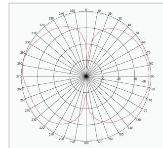
850 MHz
