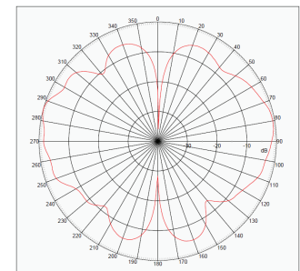
2.5 GHz
