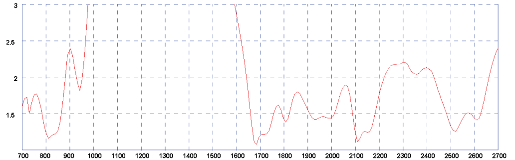
Typical VSWR*
