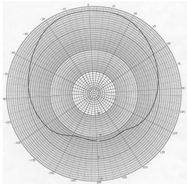
2500 MHz Elevation Plot
