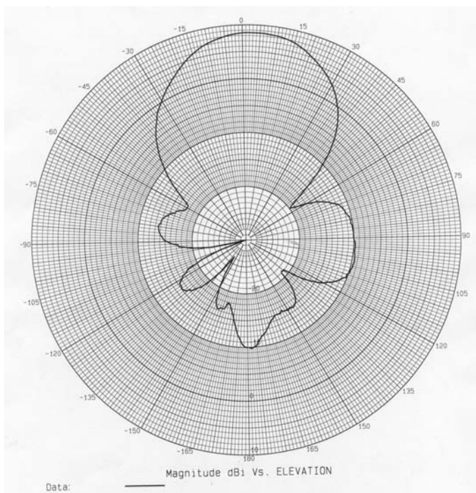
5100 MHz Elevation Plot
