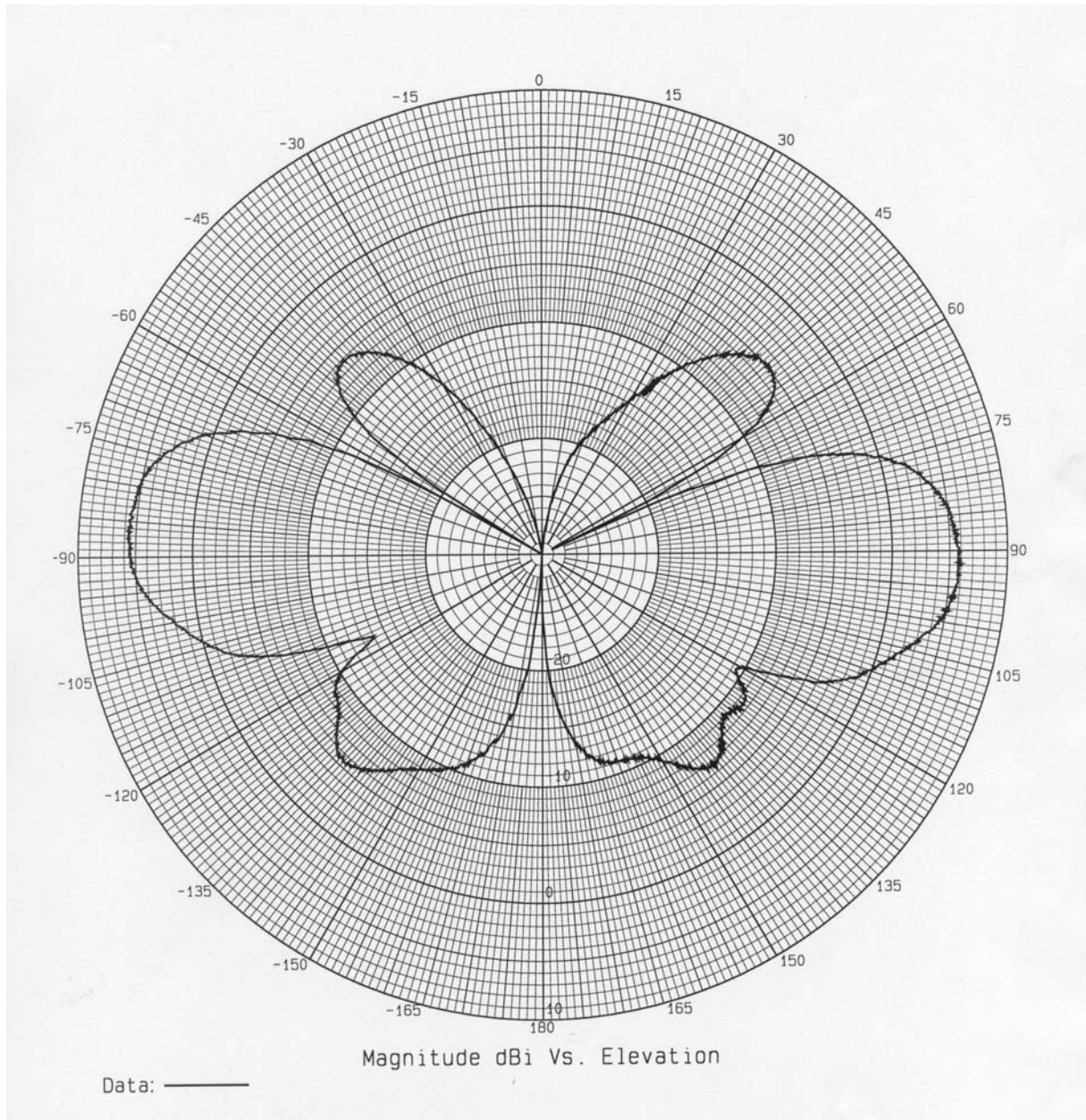
ECOS6-2600 Series – Elevation Plot
